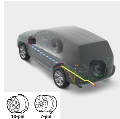
Art.-Nr. 99002-53Z00-030 (E-kit 13-pin) Art.-Nr. 99002-53Z00-022 (Fitting kit for E-kit 13-pin) E-Satz, 13-polig.
